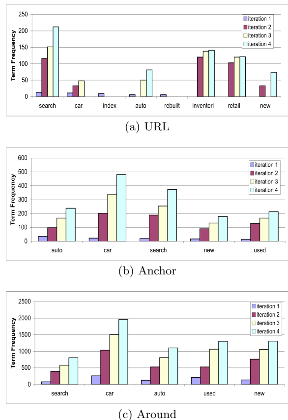
Figure 6: Features automatically extracted in different iterations of adaptive learning for Online in the Auto domain.
