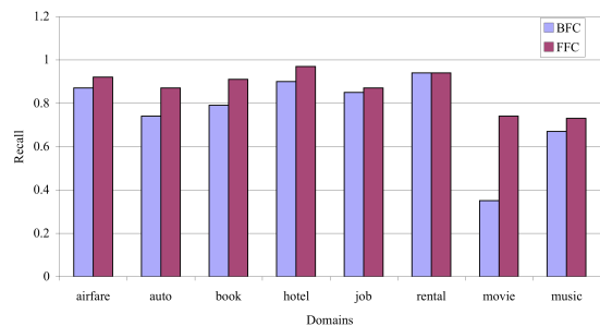
(c) Recall
