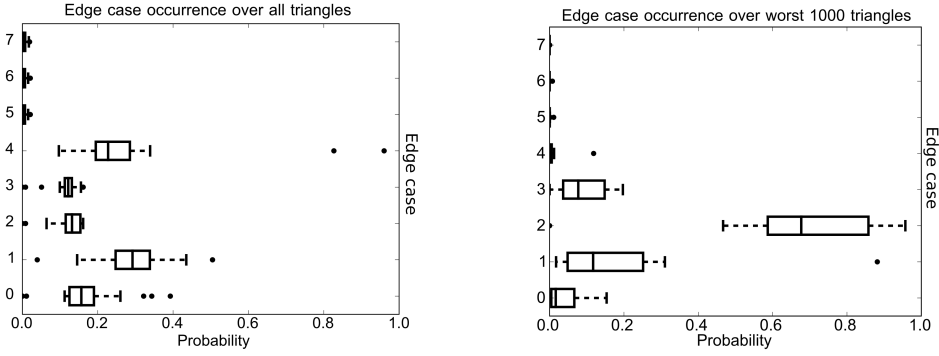
Fig. 3. Box plots show the edge group distribution for 30 different datasets collected by [6]. The left plot shows the overall distribution of edge cases for the datasets, and the right plot shows the distribution of the worst 1000 triangles. Notice that case 2 dominates the bad triangles.
