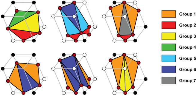
Fig. 4. Replacing cases in MC. The top row shows the original triangulation in 3 MC cases (case 5, complement of case 6 and case 11, respectively [18]), while the bottom row shows the modified connectivity. The reconnection of the cut points removes the edge group 2 from these cells, reducing the probability of generating low quality triangles.
