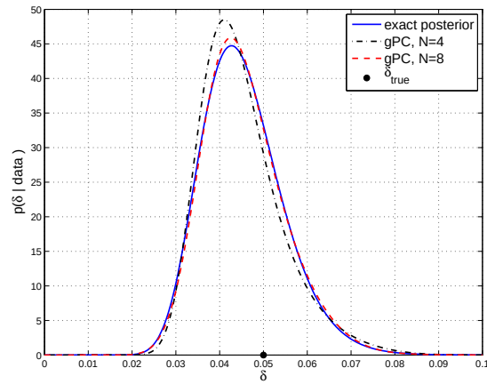
(b) \nu = 0.10 .
