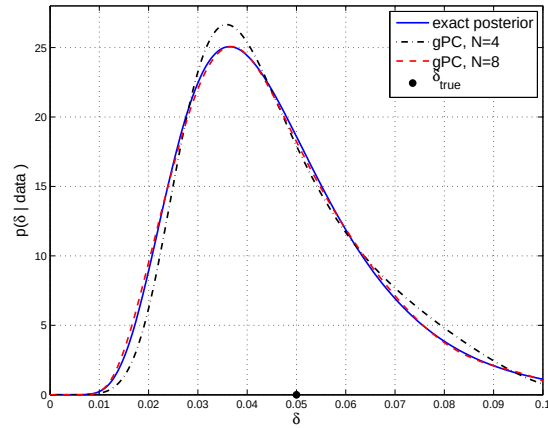
(a) \nu = 0.05 .
