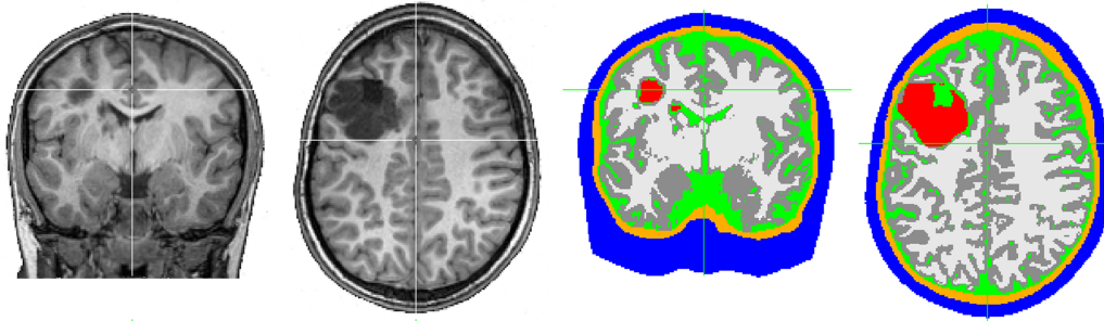
Figure 1. Coronal and axial view of the T1-MRI (left) and the corresponding segmentation (right) with six tissue types: red indicates the lesion, dark gray the gray matter, light gray the white matter, green the CSF, orange the skull and blue indicates the skin.
