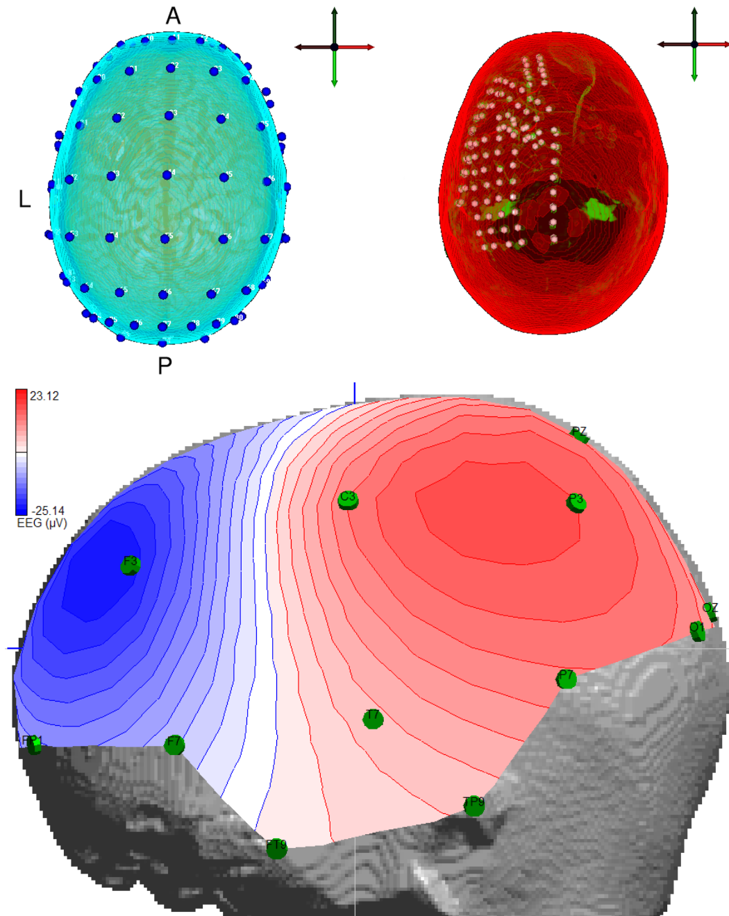
Figure 4. a) Left: The 10-10 standard system EEG electrodes (blue spheres) mapped to the head model of the patient. Right: The outermost layer of the head model (red) and a segmented part of the co-registered CT dataset (green) are shown together with the extracted and mapped iEEG electrode positions. b) EEG interpolated isopotential distribution at the signal peak.
