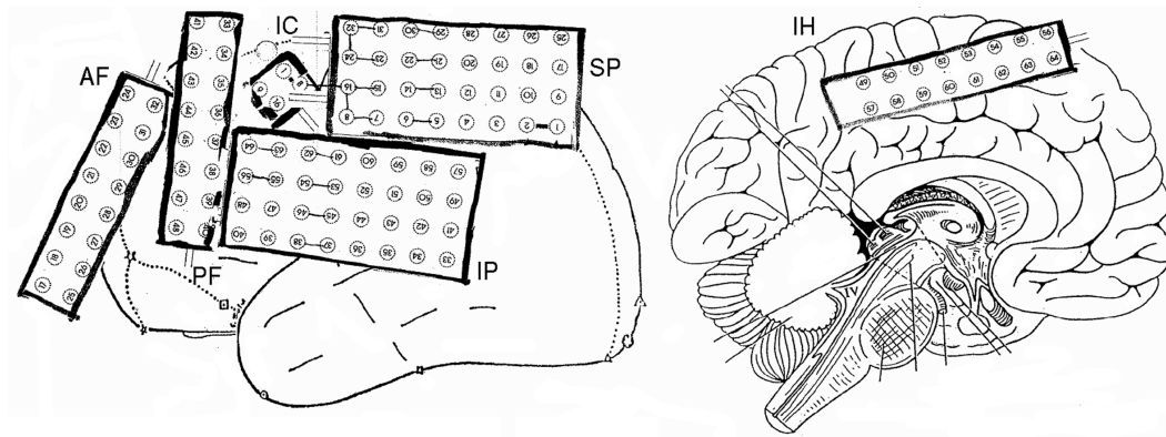
Figure 5. The positions and labels of the iEEG electrodes in the patient's record. Different stripes are shown, where AF means anterior frontal, PF posterior frontal, IC intra cavity, IP inferior parietal, SP superior parietal and IH interhemisphere.
