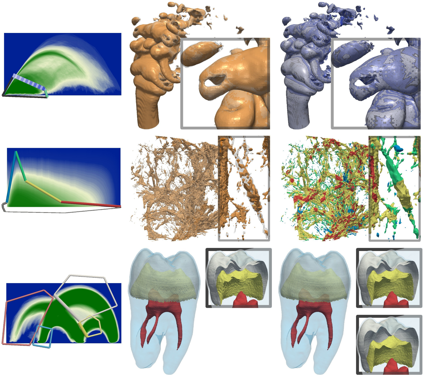
Fig. 11. Visual comparison with the raster algorithm [6]. Left: continuous scatter plot and FSCP. Center: fiber surfaces extracted with the raster algorithm. Right: fiber surfaces extracted with our algorithm.
