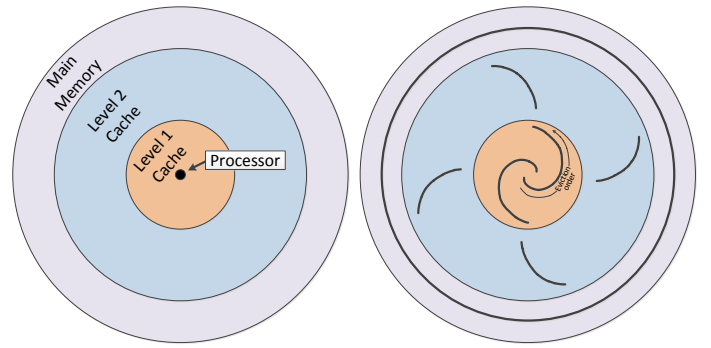
Fig. 2. Left: Our visualizations are structured schematically as concentric rings representing the main memory and levels of cache. The central point represents the CPU. Increasingly distant from the center are the L1 and L2 caches, with main memory as the farthest ring. Right: Against this backdrop, point glyphs representing data items move from place to place to indicate residency in the various levels of the memory hierarchy. In the cache levels, the glyphs arrange themselves into groupings indicating the associative cache sets, with data on the verge of eviction appearing nearer the boundaries between the levels.
