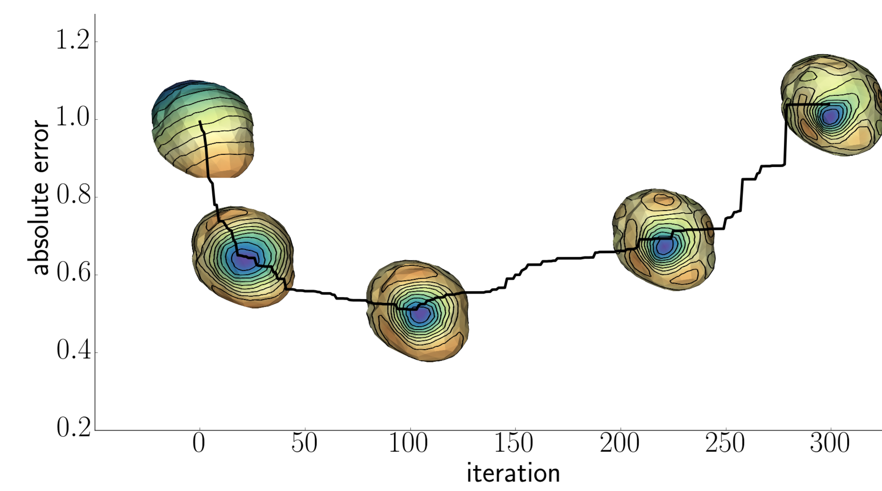
Krylov iterative regularization
