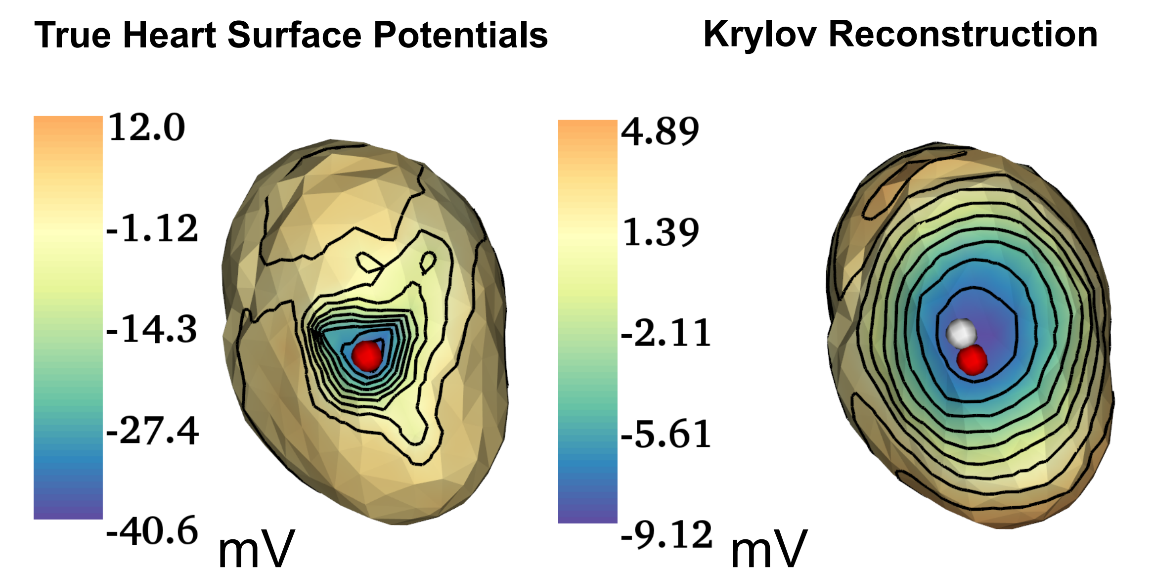
Krylov regularization for PVC localization
