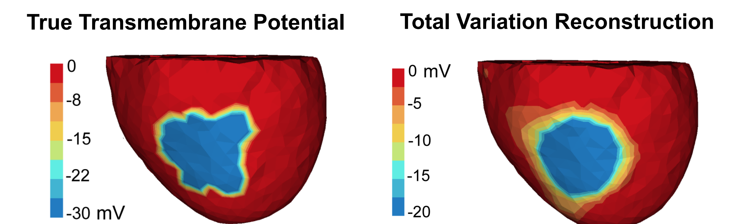
Total variation for ischemia localization
