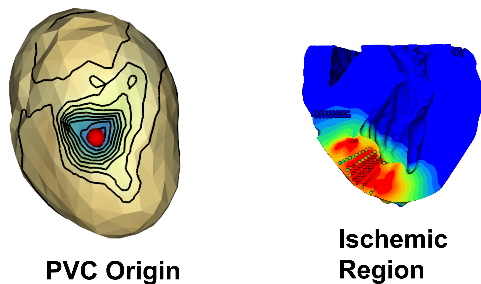
ECGI for ischemia and premature ventricular contraction (PVC)
