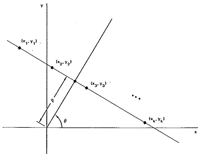
Fig. 2. Projection of colinear points onto a line.
