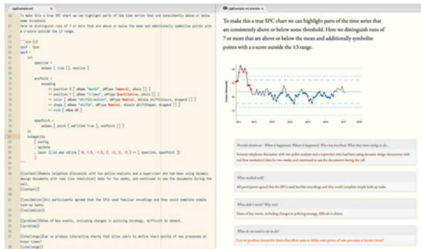
Figure 3. A screenshot from our LitVis environment showing the markdown (left) and rendering (right) of a design description and design narrative that employ an example reflective schema that requires a series of prompts for reflection.
