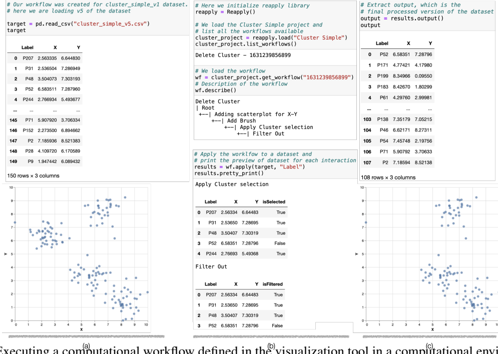
Figure 6: Executing a computational workflow defined in the visualization tool in a computational environment. (a) We first load the dataset. (b) We load the workflow library and the workflow we are interested in. We then apply the workflow to the dataset. The tool plots a preview of the actions. Note that new isSelected and isFiltered Boolean column are introduced when a brush and filter are added in the preview. (c) After the filter is applied, the number of rows is reduced from 150 to 108. A visualization of the result shows the cluster was removed. Visit the notebook .
