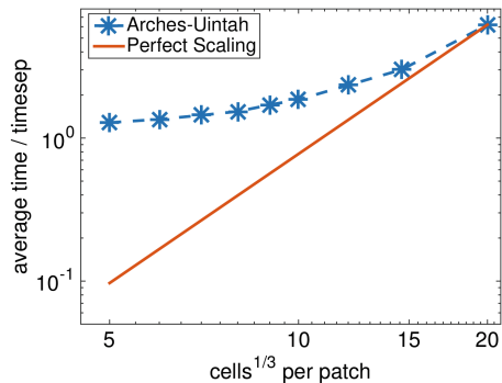
Fig. 1. Time taken for execution of a timestep for different patch sizes. Execution time starts to increase rapidly after a patch size of 12^3 .
